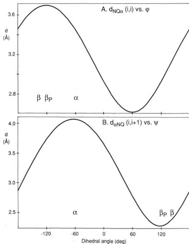
FIGURE 7: Dependence of intraresidual and sequential distances on the intervening dihedral angle in N-methylated polypeptides. (A) Intraresidual distance between the pseudatom NQ in the center of the three N-methyl protons and the C^\alpha proton, d_{NQ\alpha}(i,i) , versus \phi_i . (B) Sequential distance d_{\alpha NQ}(i,i+1) versus \psi_i . The values of \phi and \psi that correspond to a regular \alpha -helix or a parallel or antiparallel \beta -sheet are indicated by the letters \alpha , \beta_P , and \beta , respectively.
