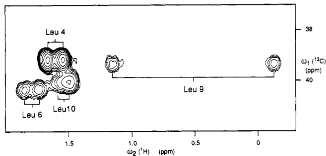
FIGURE 5: Identification of the leucine \beta -methylene groups in CsA bound to CYP in a ^{13}\text{C}, ^1\text{H} -COSY spectrum of fully ^{13}\text{C} -labeled CsA bound to unlabeled CYP. The resonance positions of the individual \beta -protons and \beta -carbons in MeLeu 4, MeLeu 6, MeLeu 9, and MeLeu 10 are indicated in the figure (0.8 mM CsA-CYP complex in 550 \mu\text{L} of ^2\text{H}_2\text{O} , 10 mM potassium deuterioacetate, 10 mM potassium phosphate, \text{pH} 6.0, 25 ^{\circ}\text{C} , ^1\text{H} frequency 500 MHz).
