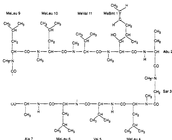
FIGURE 1: Chemical structure of cyclosporin A (CsA) with the standard numbering of the amino acid residues. Symbols: MeBmt, (4 R )-4-[( E )-2-butenyl]-4,4-dimethyl-L-threonine; Abu, L- \alpha -amino-butyric acid; MeLeu, N -methylleucine; MeVal, N -methylvaline.
